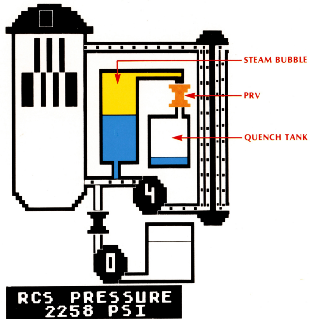
Figure 5. The Pressurizer
