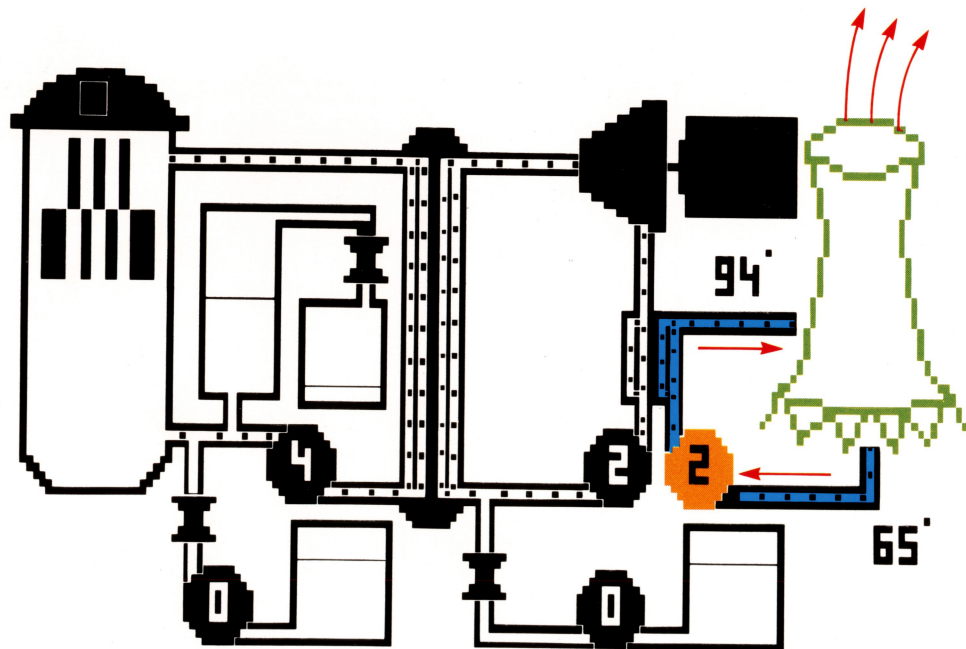
Figure 9. Cooling Tower
