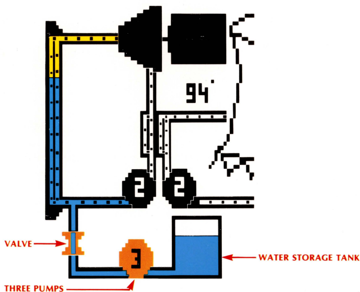
Figure 11. Auxiliary Feedwater System
