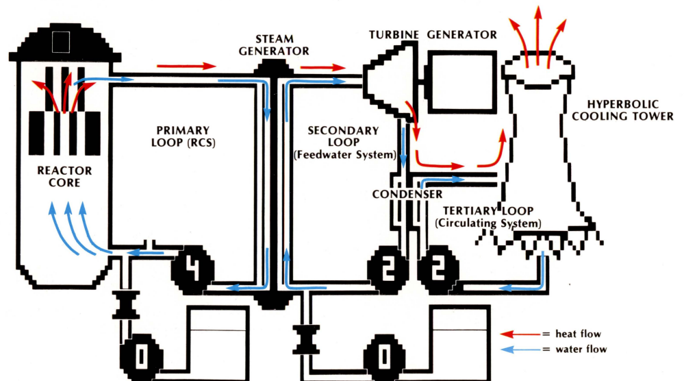
Figure 1. Heat Transfer in the PWR System
