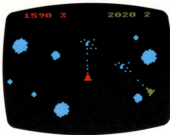
Figure 11. ASTERIODS in Play
